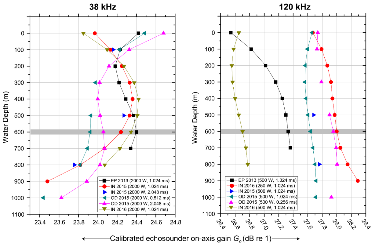
Figure 2. Represents depth-dependent repeatability in calibrated G_0 over the calibration deployments.
